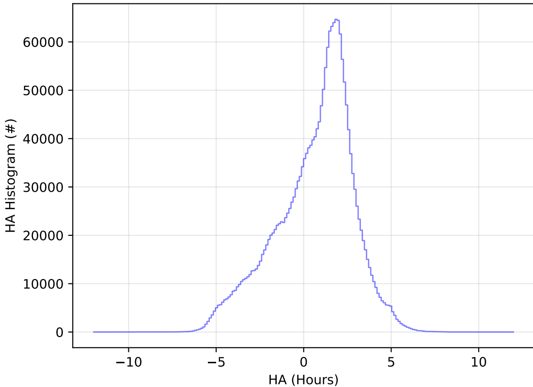
too_elab_2yr_r64_d3_ugrizy_v3.4_10yrs WFD all bands: HA Histogram
