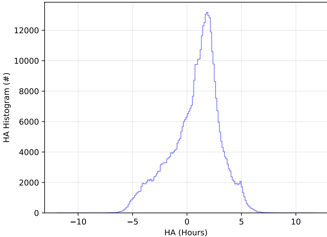
too_elab_2yr_r64_d3_ugrizy_v3.4_10yrs All sky z band: HA Histogram
