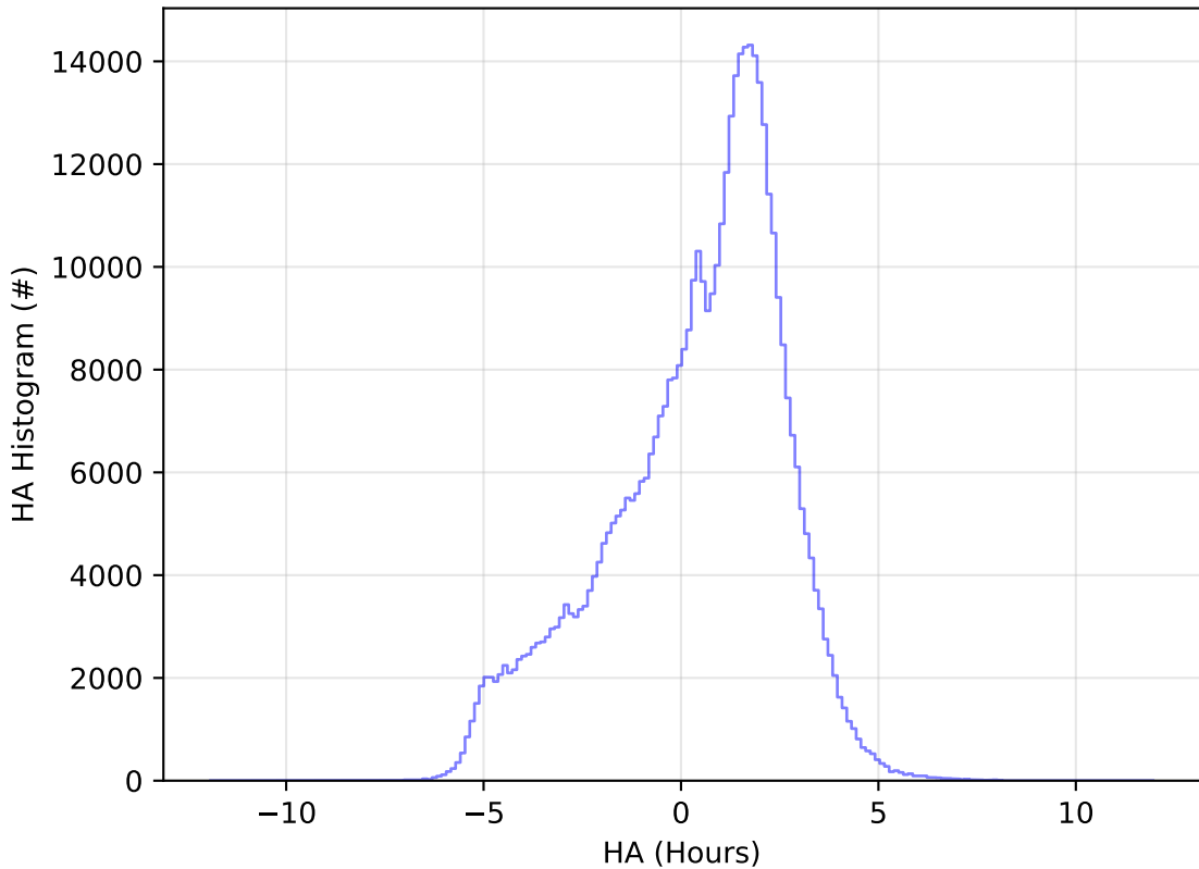
too_elab_2yr_r64_d3_ugrizy_v3.4_10yrs All sky r band: HA Histogram
