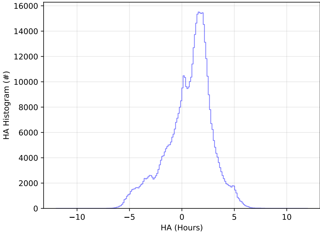
too_elab_2yr_r64_d3_ugrizy_v3.4_10yrs All sky i band: HA Histogram
