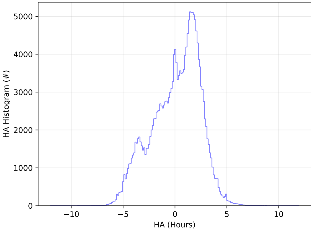
too_elab_2yr_r64_d3_ugrizy_v3.4_10yrs All sky g band: HA Histogram
