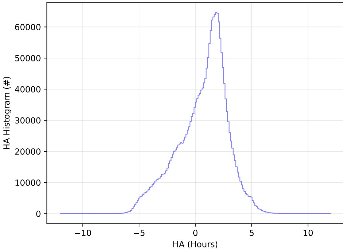
too_elab_2yr_r64_d3_ugrizy_v3.4_10yrs All sky all bands: HA Histogram
