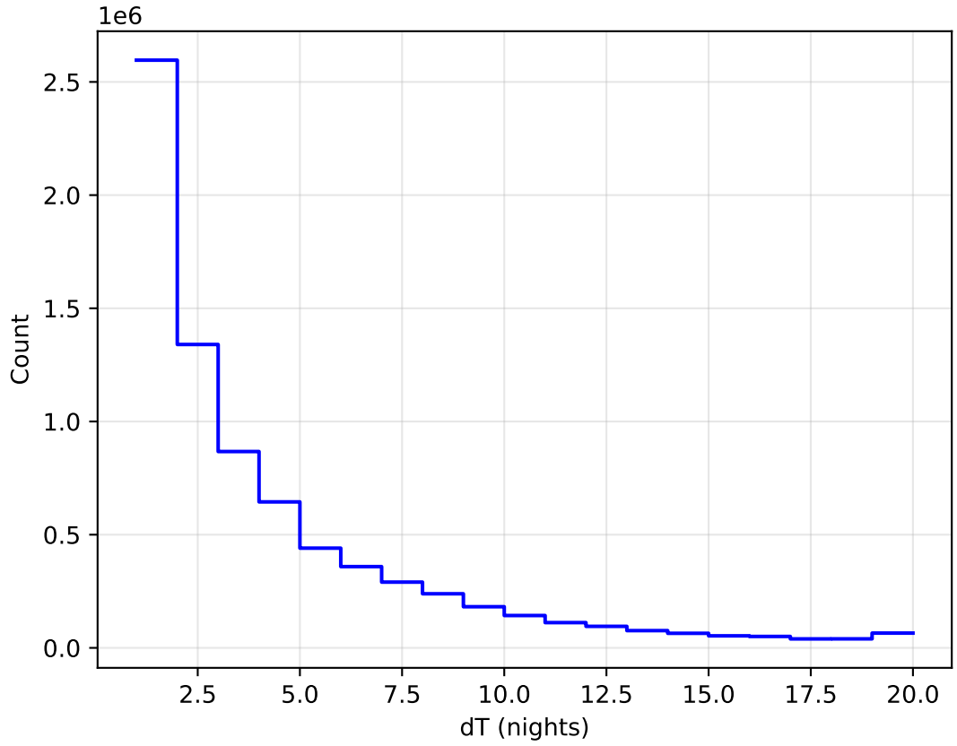
too_elab_2yr_r64_d3_ugrizy_v3.4_10yrs WFD all bands: DeltaNight Histogram
