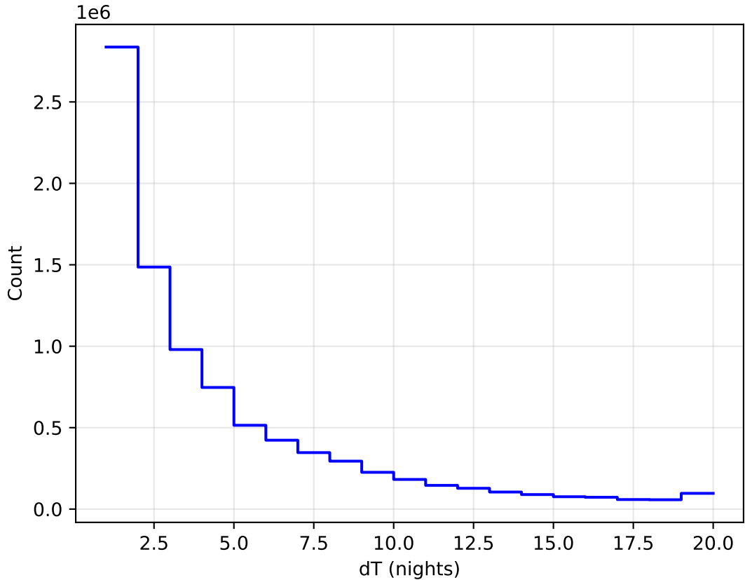
too_elab_2yr_r64_d3_ugrizy_v3.4_10yrs All sky all bands: DeltaNight Histogram
