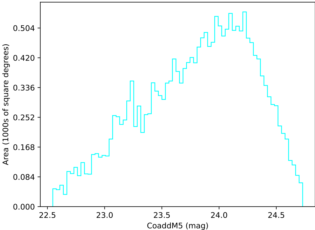
too_elab_2yr_r64_d3_ugrizy_v3.4_10yrs Yr 3-4 u band: CoaddM5
