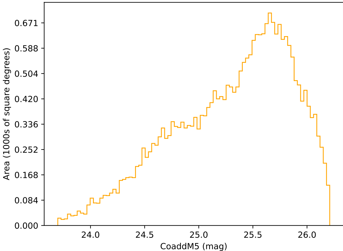
too_elab_2yr_r64_d3_ugrizy_v3.4_10yrs Yr 3-4 r band: CoaddM5
