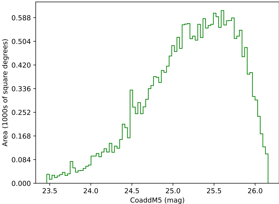
too_elab_2yr_r64_d3_ugrizy_v3.4_10yrs Yr 3-4 g band: CoaddM5
