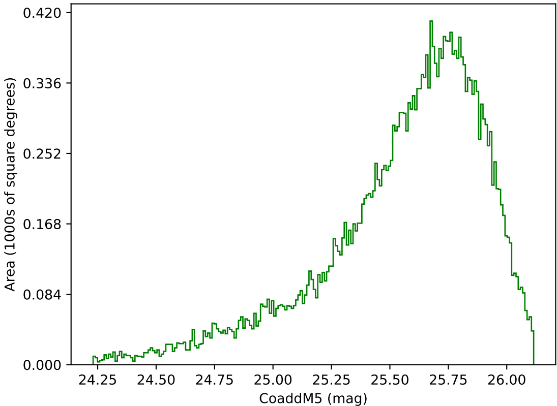
too_elab_2yr_r64_d3_ugrizy_v3.4_10yrs Yr 1 g band: CoaddM5
