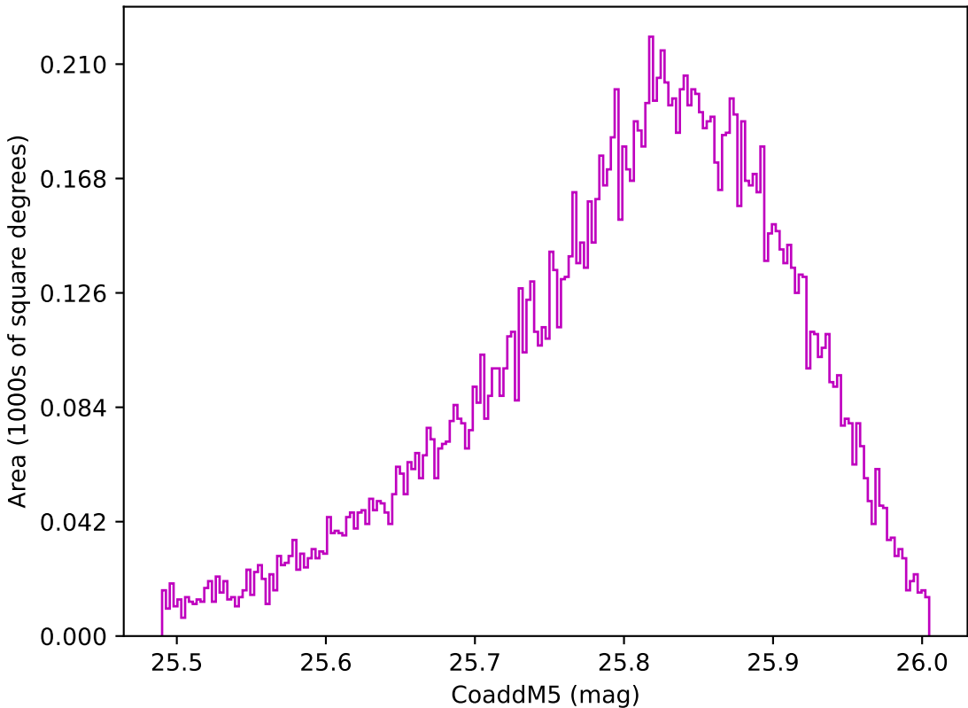
too_elab_2yr_r64_d3_ugrizy_v3.4_10yrs WFD z band: CoaddM5
