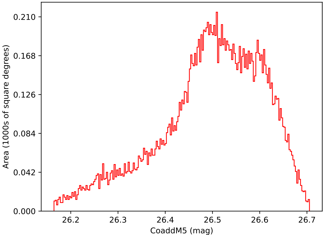
too_elab_2yr_r64_d3_ugrizy_v3.4_10yrs WFD i band: CoaddM5
