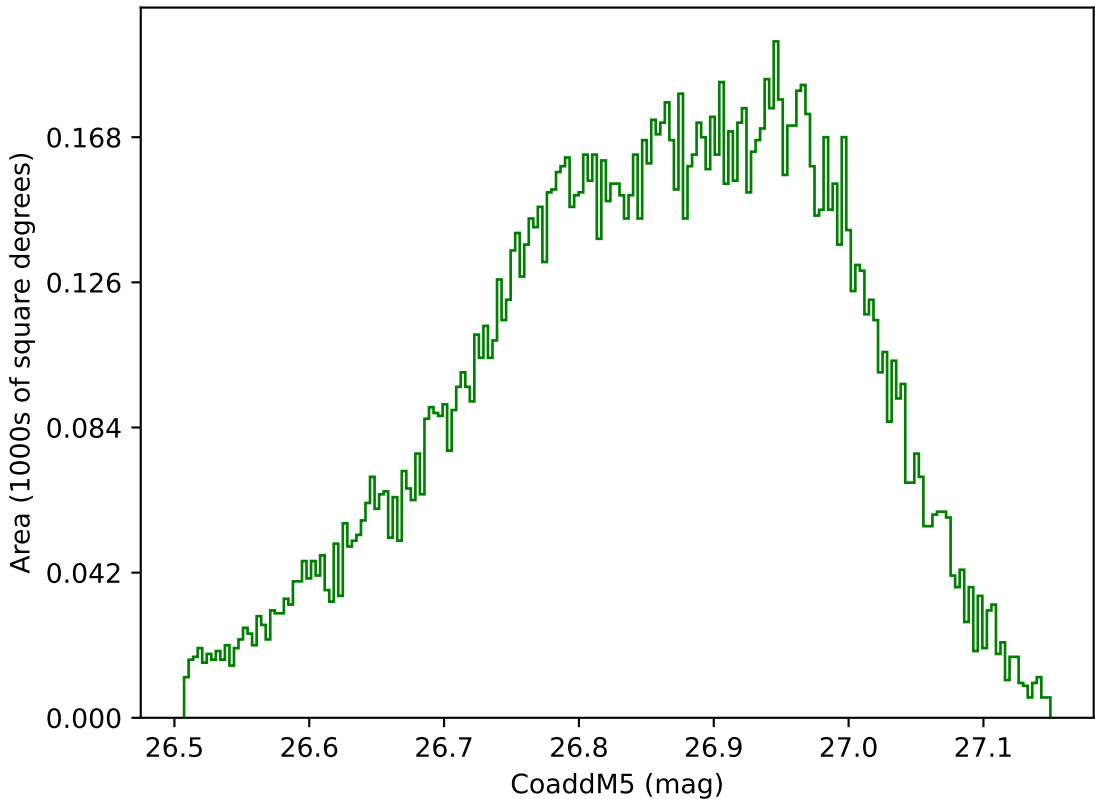
too_elab_2yr_r64_d3_ugrizy_v3.4_10yrs WFD g band: CoaddM5
