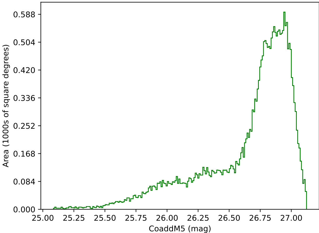
too_elab_2yr_r64_d3_ugrizy_v3.4_10yrs All sky g band: CoaddM5
