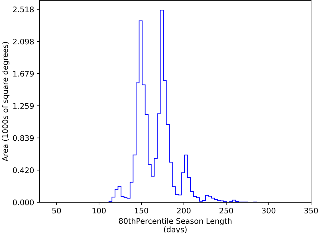
too_elab_2yr_r64_d3_ugrizy_v3.4_10yrs WFD y band: 80thPercentile Season Length
