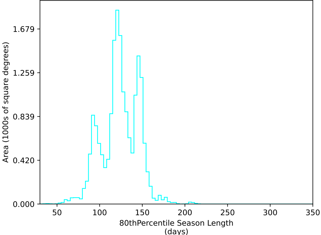
too_elab_2yr_r64_d3_ugrizy_v3.4_10yrs WFD u band: 80thPercentile Season Length
