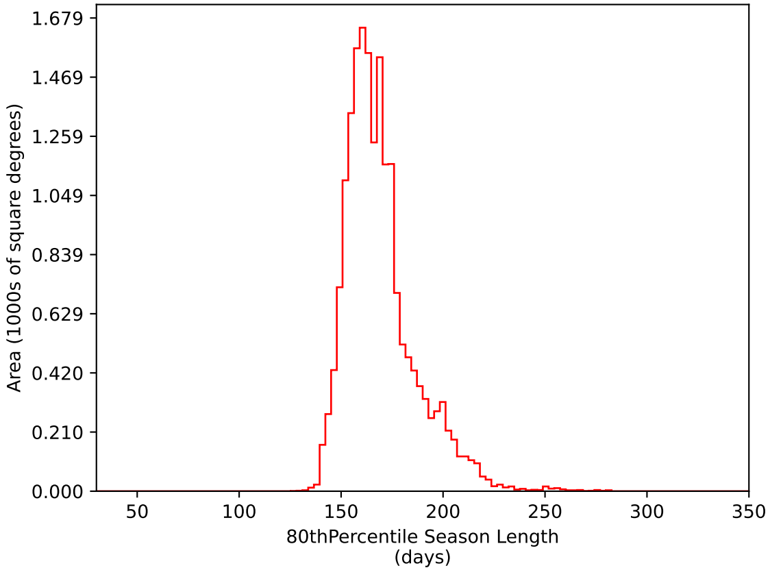
too_elab_2yr_r64_d3_ugrizy_v3.4_10yrs WFD i band: 80thPercentile Season Length
