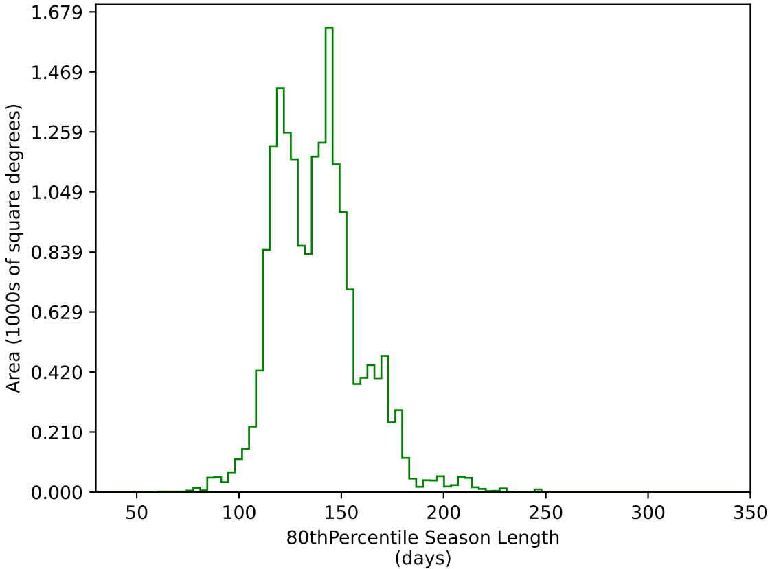
too_elab_2yr_r64_d3_ugrizy_v3.4_10yrs WFD g band: 80thPercentile Season Length
