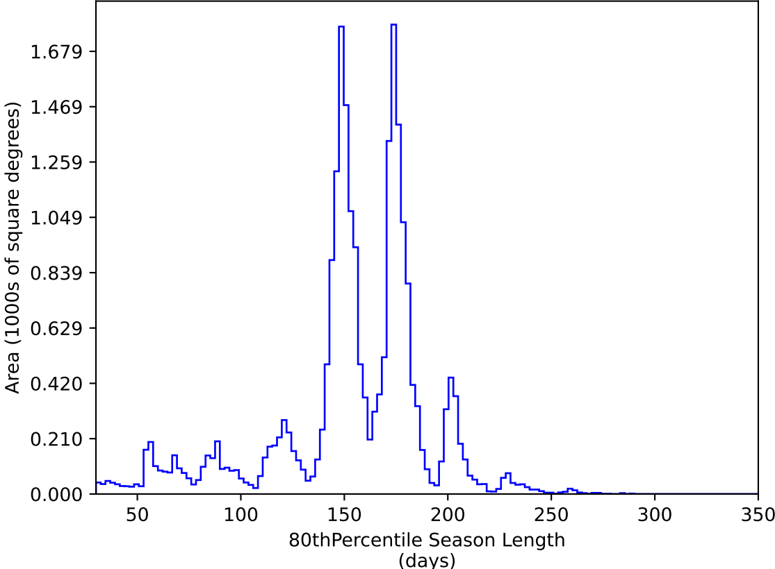
too_elab_2yr_r64_d3_ugrizy_v3.4_10yrs All sky y band: 80thPercentile Season Length
