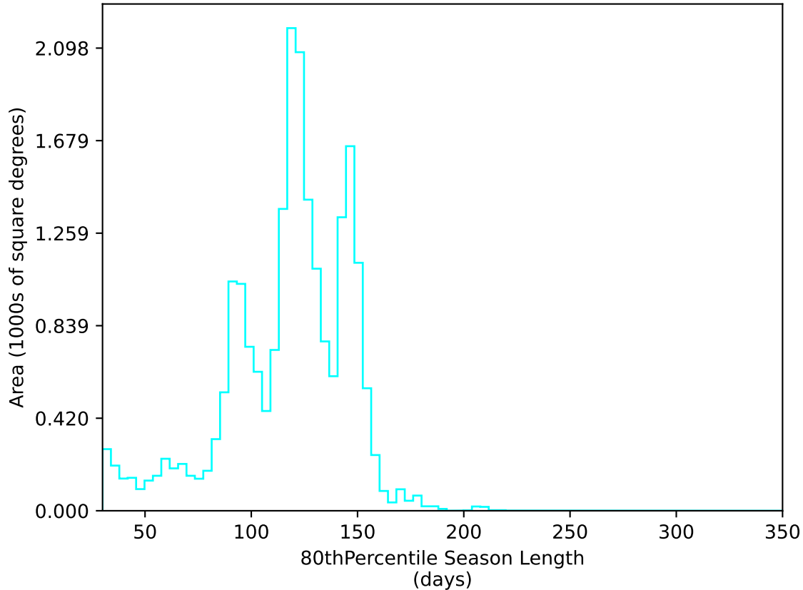
too_elab_2yr_r64_d3_ugrizy_v3.4_10yrs All sky u band: 80thPercentile Season Length
