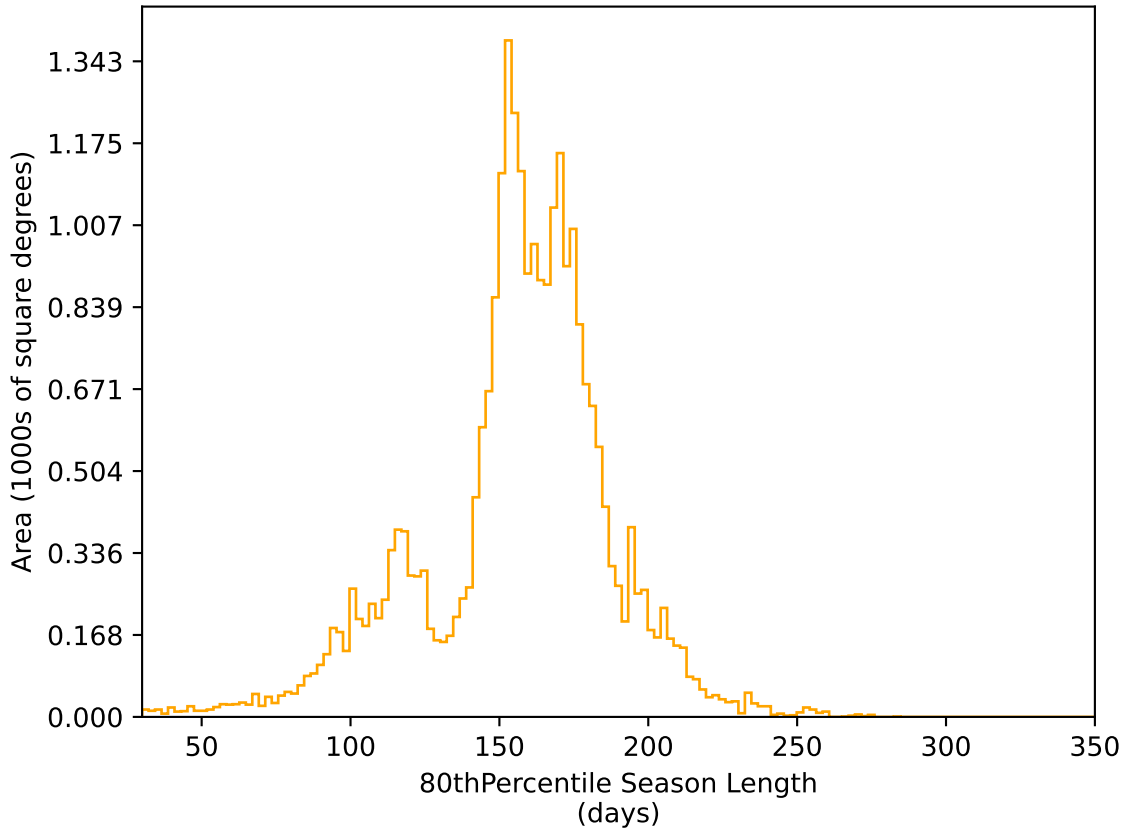
too_elab_2yr_r64_d3_ugrizy_v3.4_10yrs All sky r band: 80thPercentile Season Length
