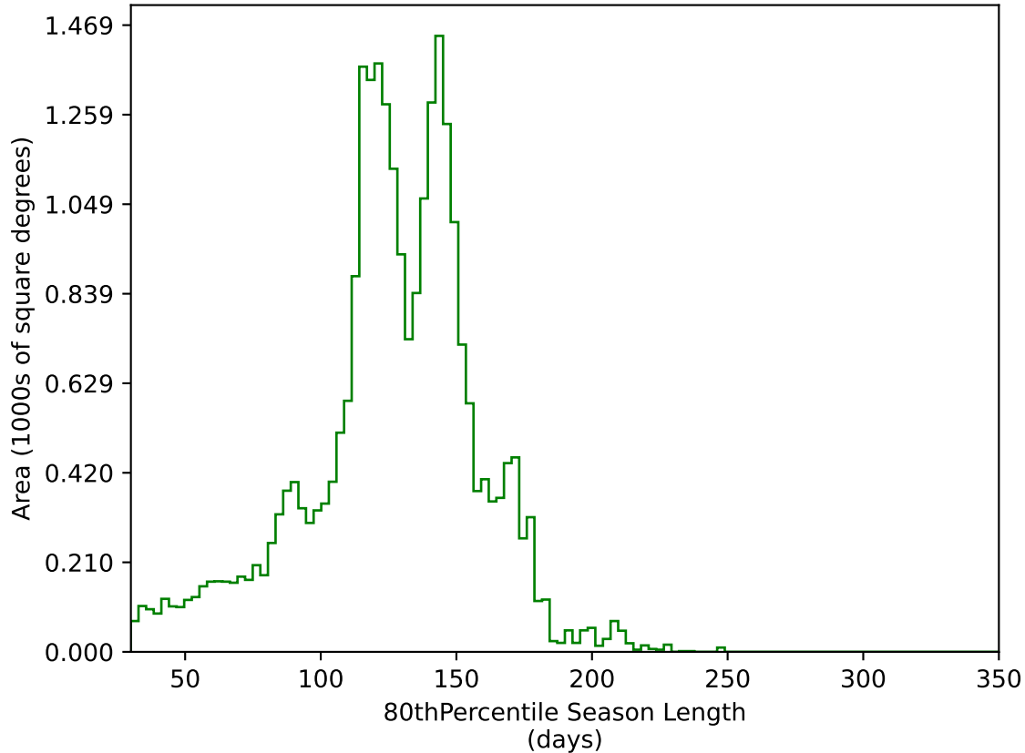
too_elab_2yr_r64_d3_ugrizy_v3.4_10yrs All sky g band: 80thPercentile Season Length
