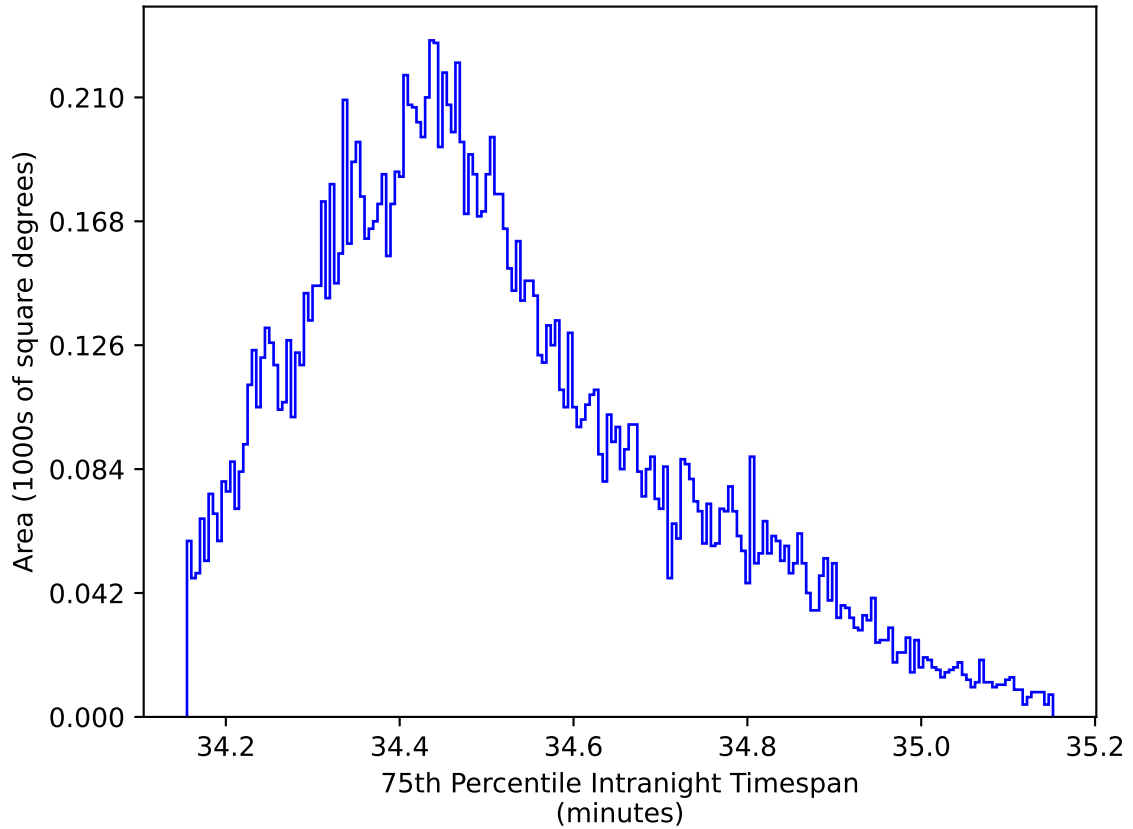
too_elab_2yr_r64_d3_ugrizy_v3.4_10yrs WFD zy bands: 75th Percentile Intranight Timespan
