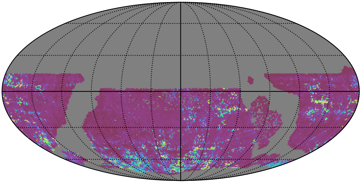
too_elab_2yr_r64_d3_ugrizy_v3.4_10yrs WFD z band: 75th Percentile Intranight Timespan
