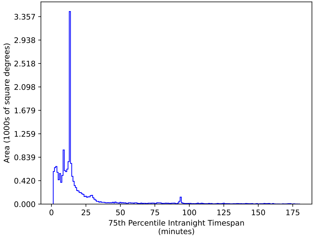
too_elab_2yr_r64_d3_ugrizy_v3.4_10yrs WFD z band: 75th Percentile Intranight Timespan
