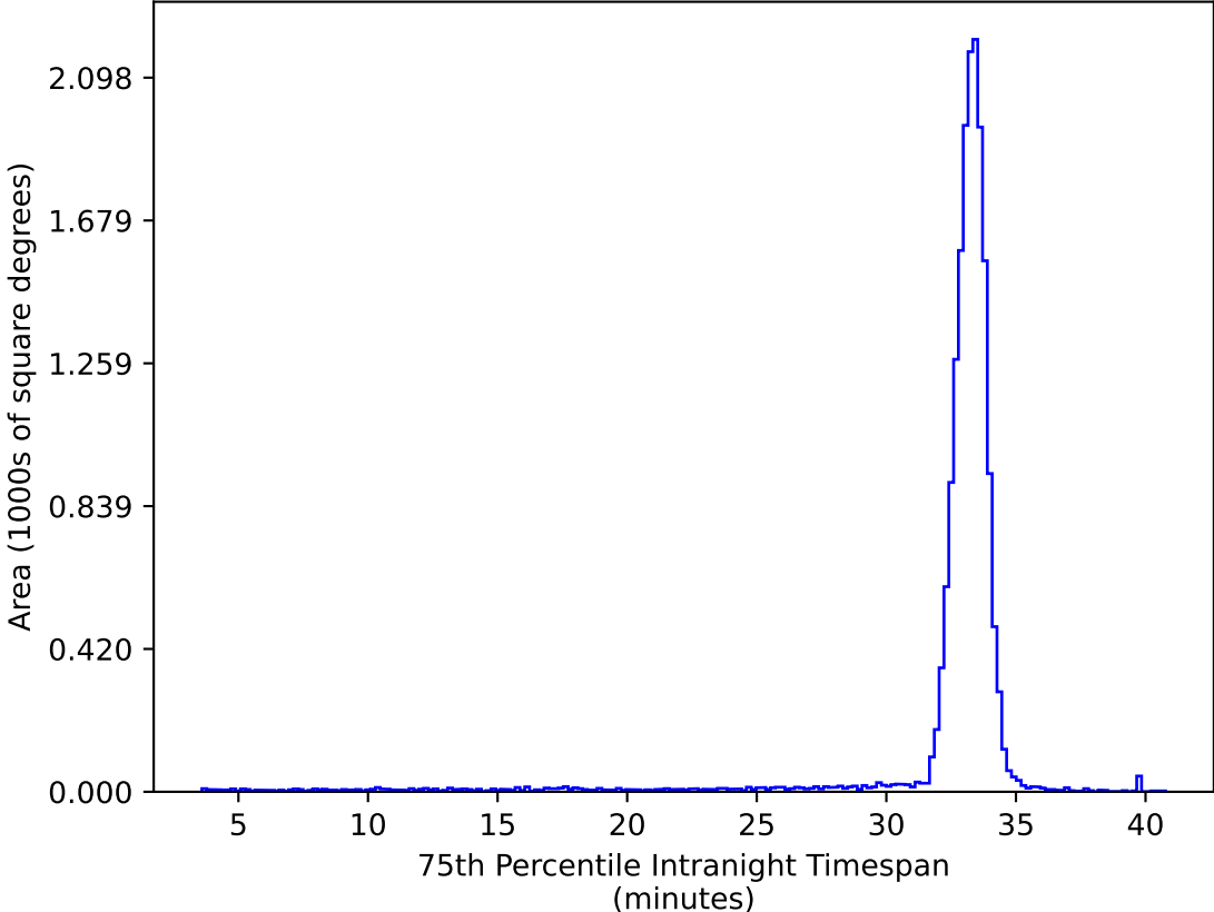
too_elab_2yr_r64_d3_ugrizy_v3.4_10yrs WFD ug bands: 75th Percentile Intranight Timespan
