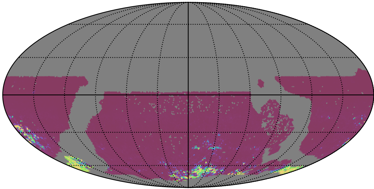
too_elab_2yr_r64_d3_ugrizy_v3.4_10yrs WFD ri bands: 75th Percentile Intranight Timespan
