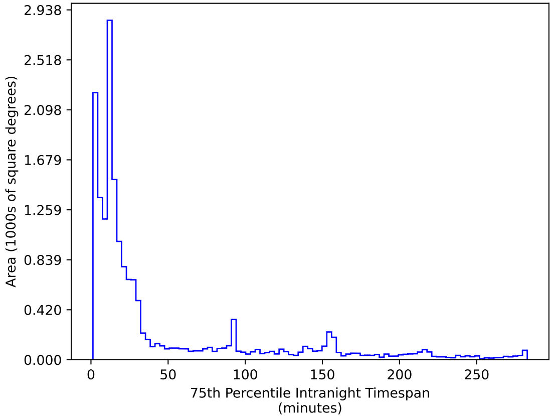
too_elab_2yr_r64_d3_ugrizy_v3.4_10yrs WFD r band: 75th Percentile Intranight Timespan
