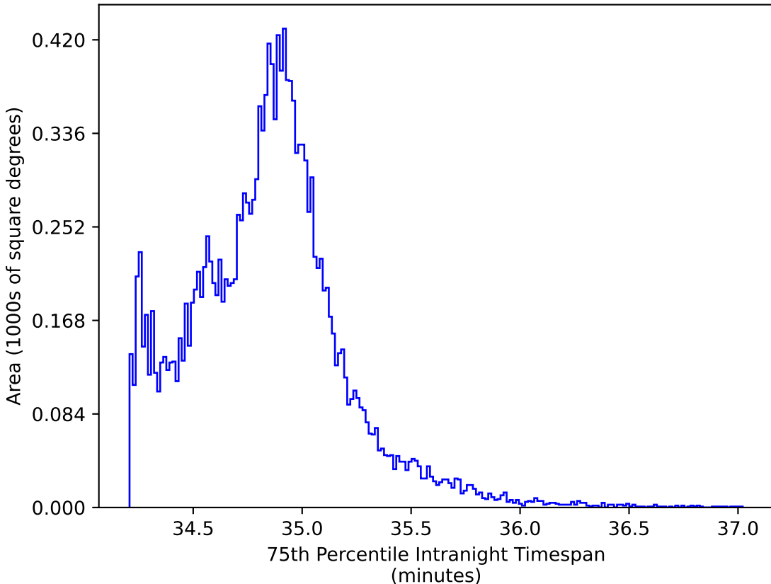
too_elab_2yr_r64_d3_ugrizy_v3.4_10yrs WFD iz bands: 75th Percentile Intranight Timespan
