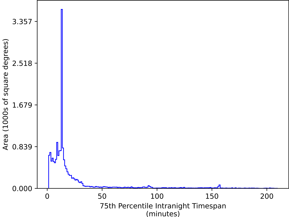
too_elab_2yr_r64_d3_ugrizy_v3.4_10yrs WFD i band: 75th Percentile Intranight Timespan
