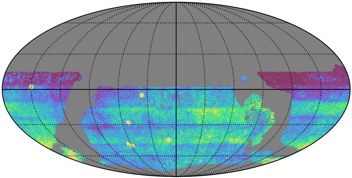
too_elab_2yr_r64_d3_ugrizy_v3.4_10yrs WFD all bands: 75th Percentile Intranight Timespan
