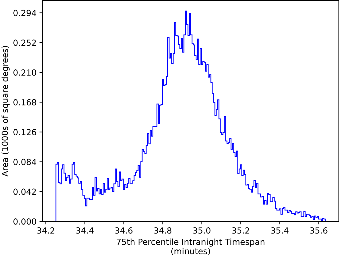
too_elab_2yr_r64_d3_ugrizy_v3.4_10yrs WFD all bands: 75th Percentile Intranight Timespan
