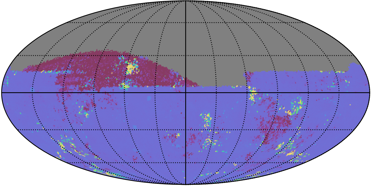
too_elab_2yr_r64_d3_ugrizy_v3.4_10yrs All sky ug bands: 75th Percentile Intranight Timespan
