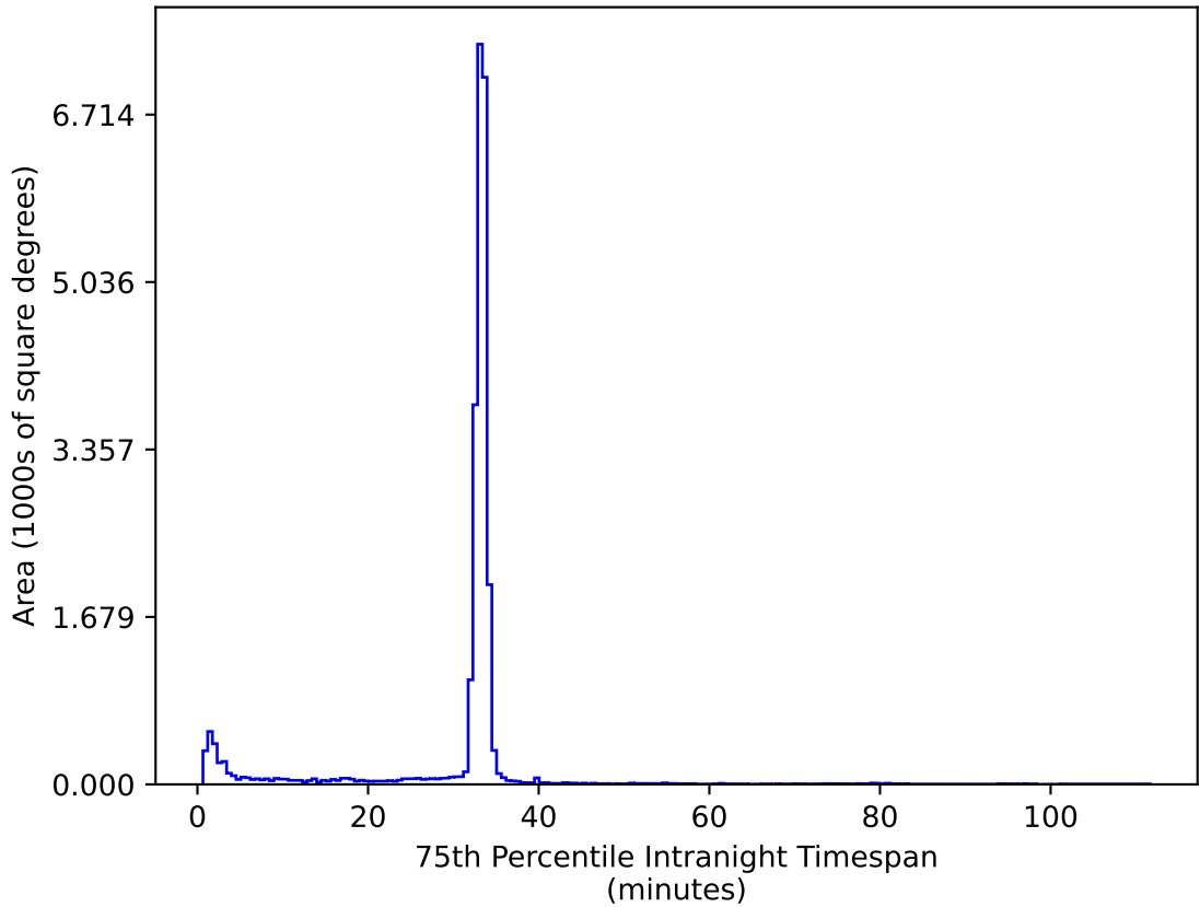
too_elab_2yr_r64_d3_ugrizy_v3.4_10yrs All sky ug bands: 75th Percentile Intranight Timespan
