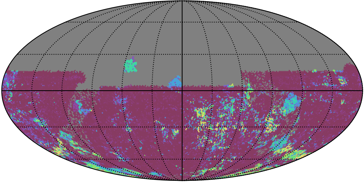
too_elab_2yr_r64_d3_ugrizy_v3.4_10yrs All sky u band: 75th Percentile Intranight Timespan
