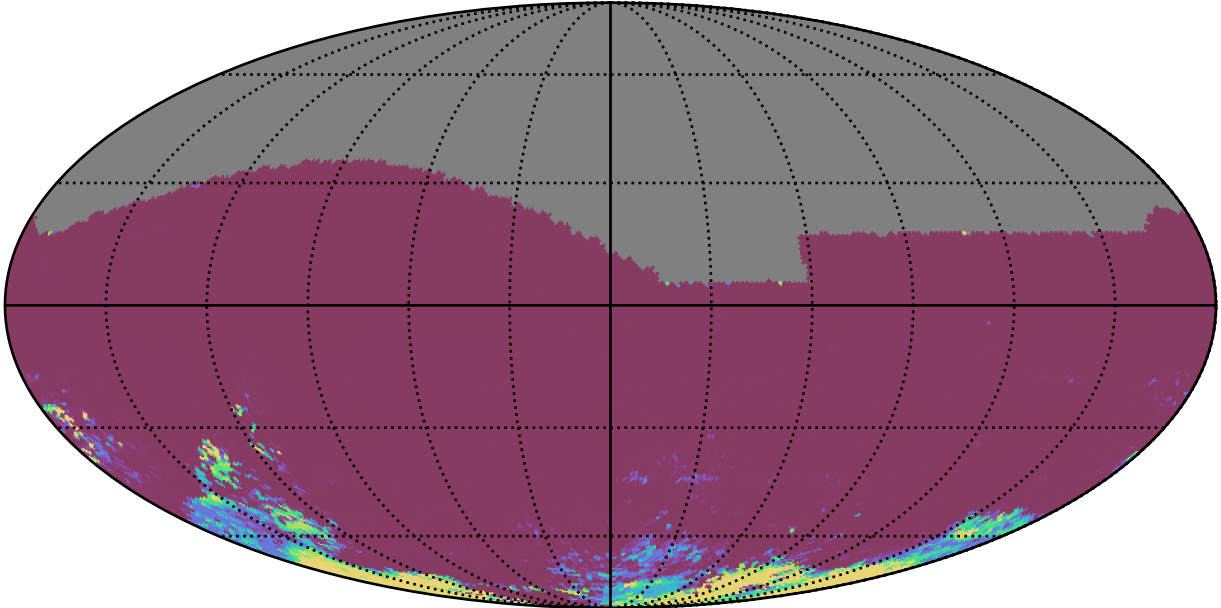
too_elab_2yr_r64_d3_ugrizy_v3.4_10yrs All sky ri bands: 75th Percentile Intranight Timespan
