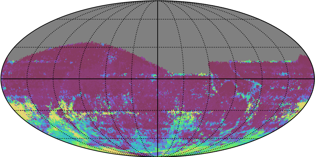
too_elab_2yr_r64_d3_ugrizy_v3.4_10yrs All sky r band: 75th Percentile Intranight Timespan
