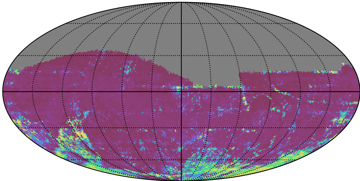
too_elab_2yr_r64_d3_ugrizy_v3.4_10yrs All sky i band: 75th Percentile Intranight Timespan
