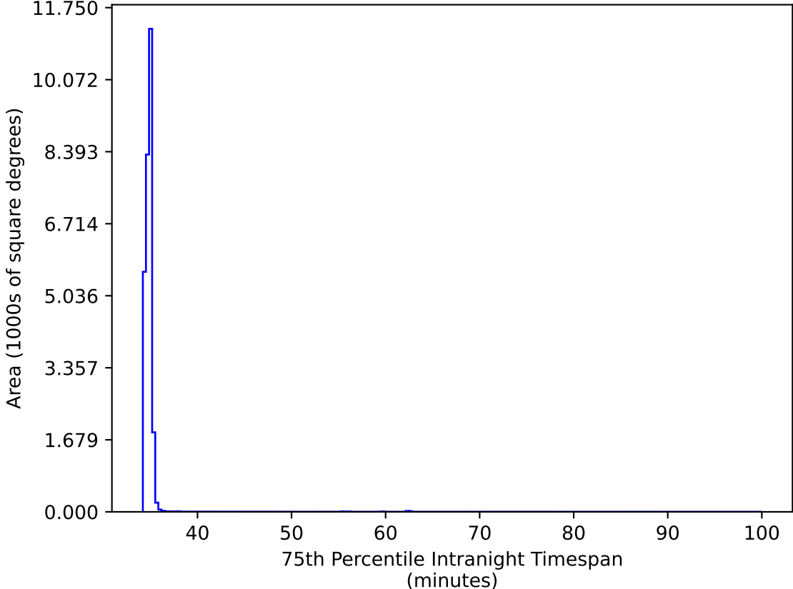
too_elab_2yr_r64_d3_ugrizy_v3.4_10yrs All sky all bands: 75th Percentile Intranight Timespan
