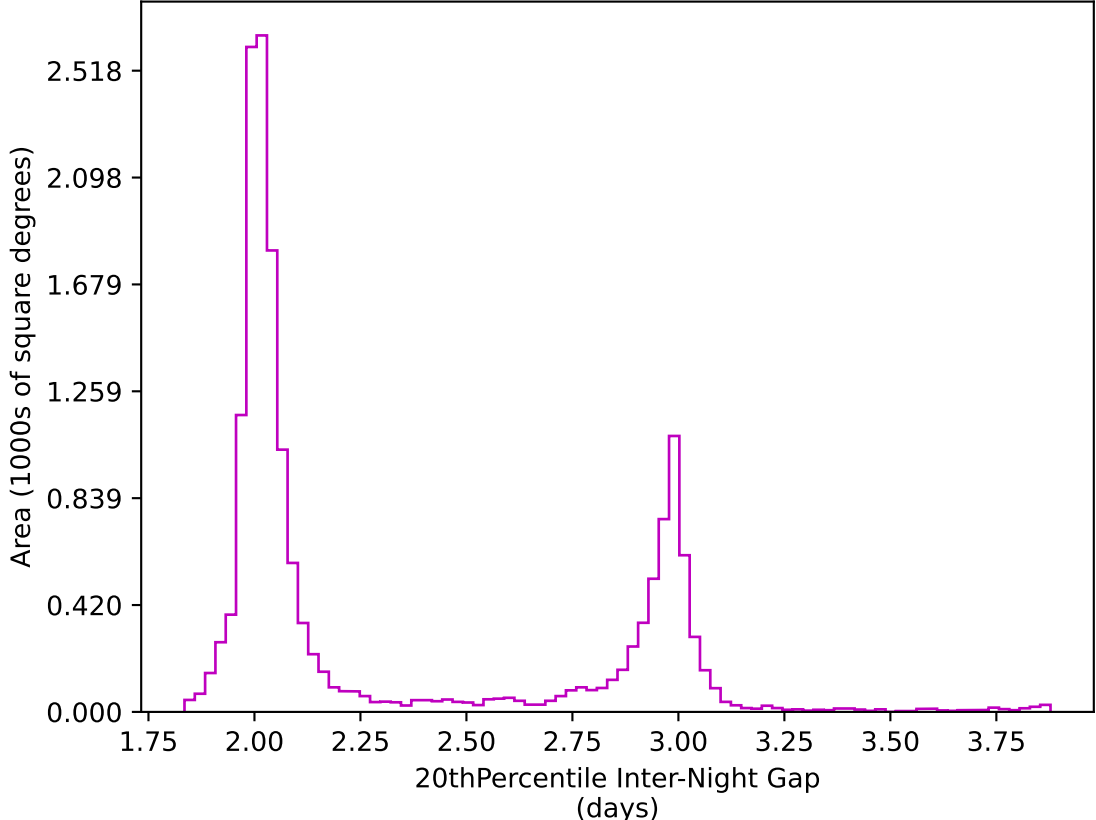
too_elab_2yr_r64_d3_ugrizy_v3.4_10yrs WFD z band: 20thPercentile Inter-Night Gap
