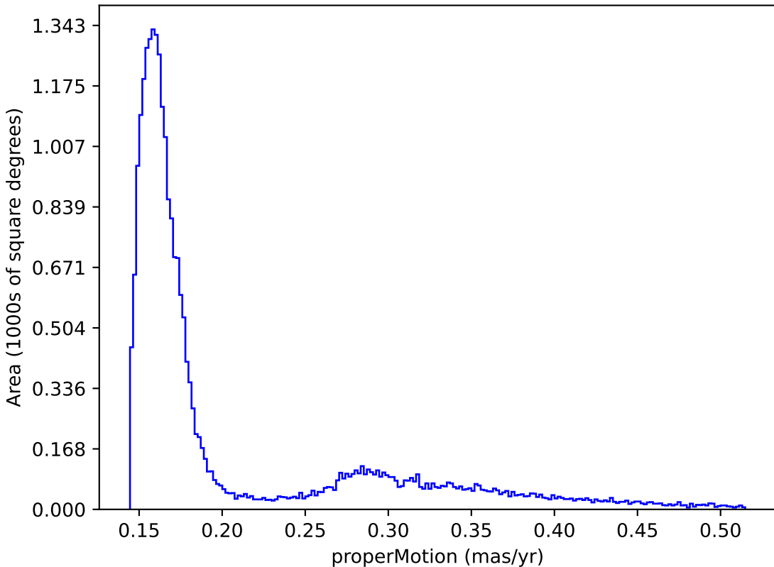
too_elab_2yr_r64_d3_ugrizy_v3.4_10yrs : properMotion
