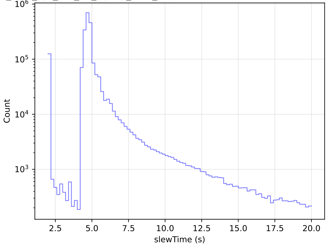
too_elab_2yr_r64_d3_ugrizy_v3.4_10yrs All visits: Zoom Slew Time Histogram
