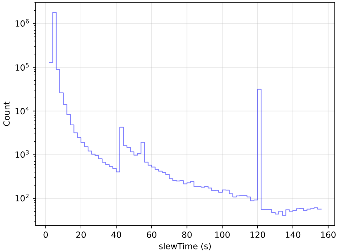
too_elab_2yr_r64_d3_ugrizy_v3.4_10yrs All visits: Slew Time Histogram
