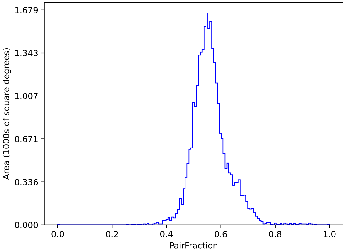
too_elab_2yr_r64_d3_ugrizy_v3.4_10yrs (g or r or i): PairFraction
