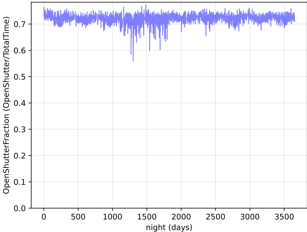
too_elab_2yr_r64_d3_ugrizy_v3.4_10yrs : OpenShutterFraction
