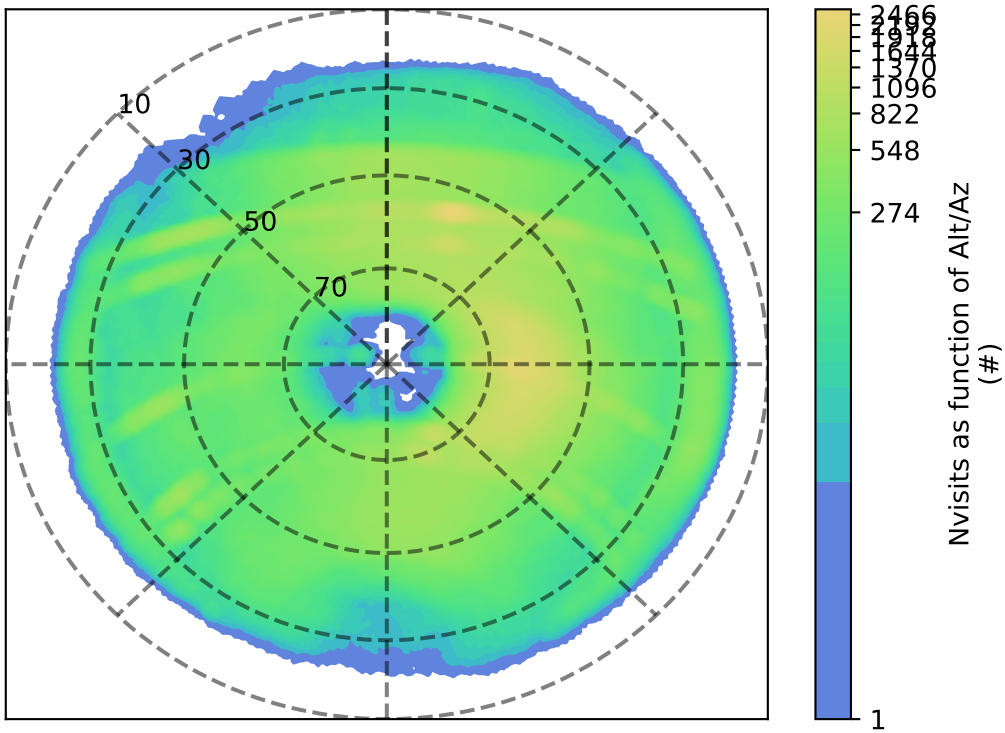
too_elab_2yr_r64_d3_ugrizy_v3.4_10yrs z: Nvisits as function of Alt/Az
