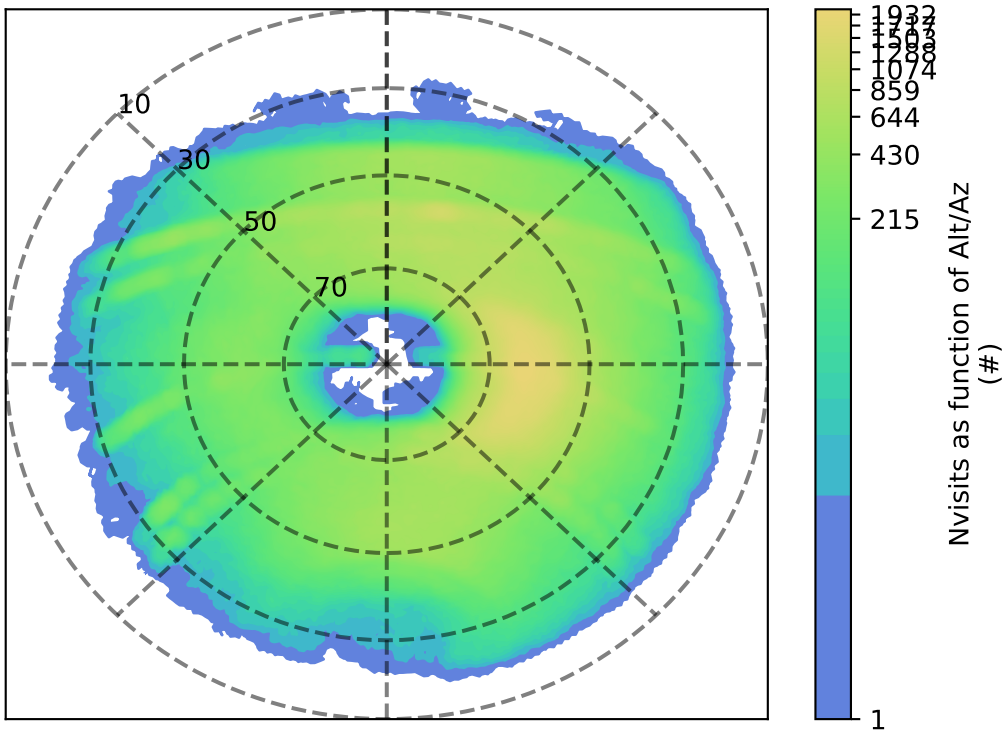
too_elab_2yr_r64_d3_ugrizy_v3.4_10yrs y: Nvisits as function of Alt/Az
