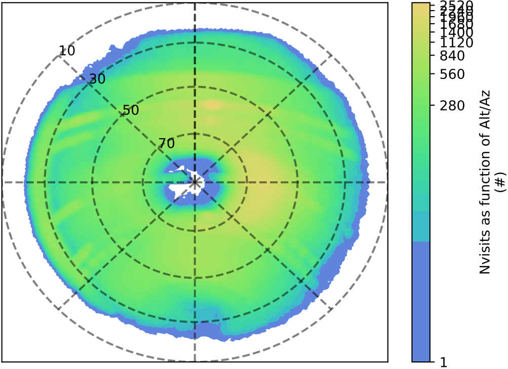
too_elab_2yr_r64_d3_ugrizy_v3.4_10yrs r: Nvisits as function of Alt/Az
